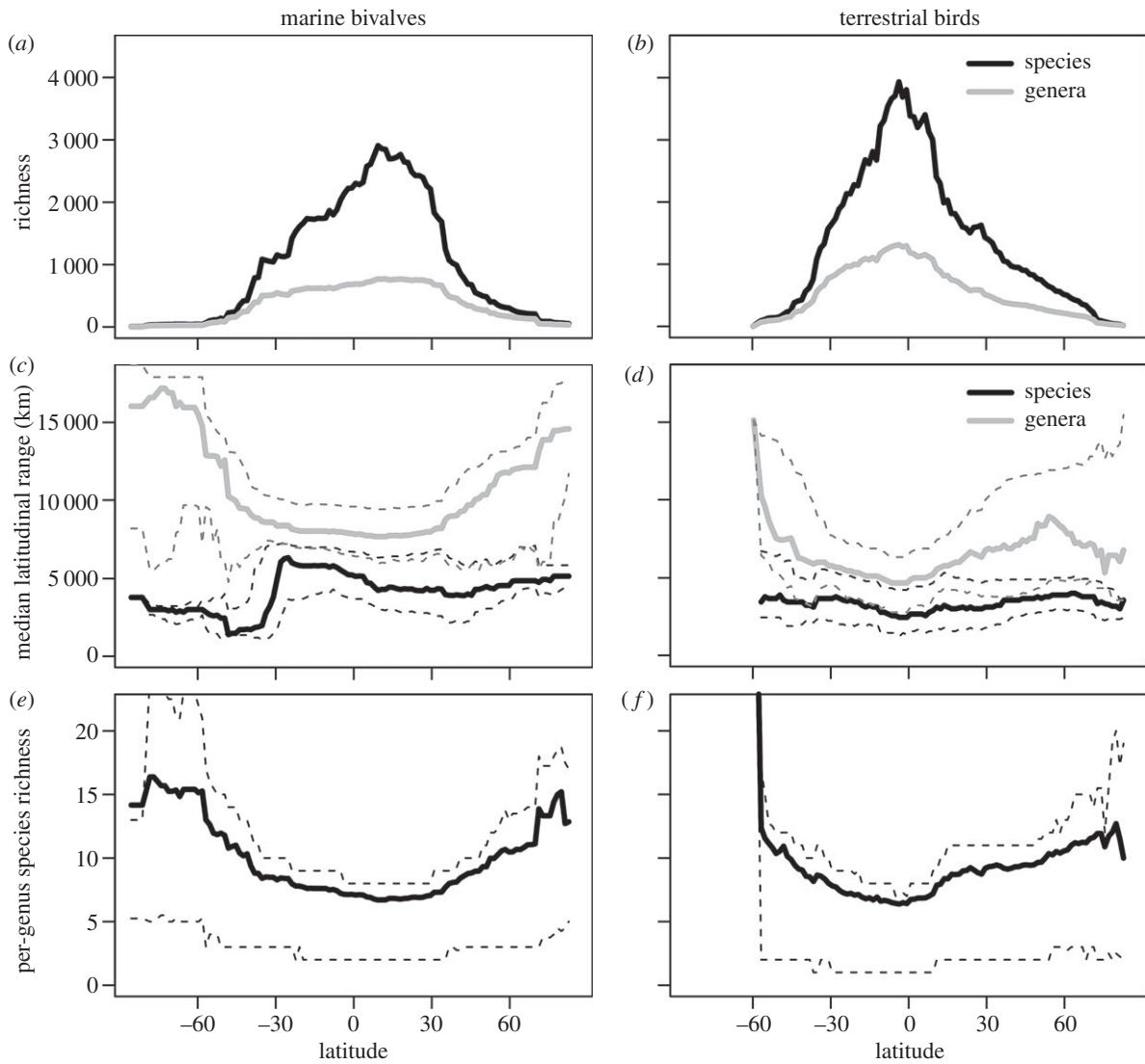
Figure 2. (a,b) Latitudinal gradients in the richness of species and genera. (c,d) Latitudinal gradients in median species and genus latitudinal range size. (e,f) Latitudinal gradients in the mean number of species within genera (species–genus ratio) that are found at a given latitude (all species in each genus are tallied, not just the species at a given latitude). All figures are plotted at the resolution of 1^\circ latitudinal bands. Dashed lines represent 25th and 75th percentiles of underlying range-size frequency distributions and per-genus richness frequency distributions. Latitudinal gradients in per-genus species richness are markedly congruent between bivalves and birds.
